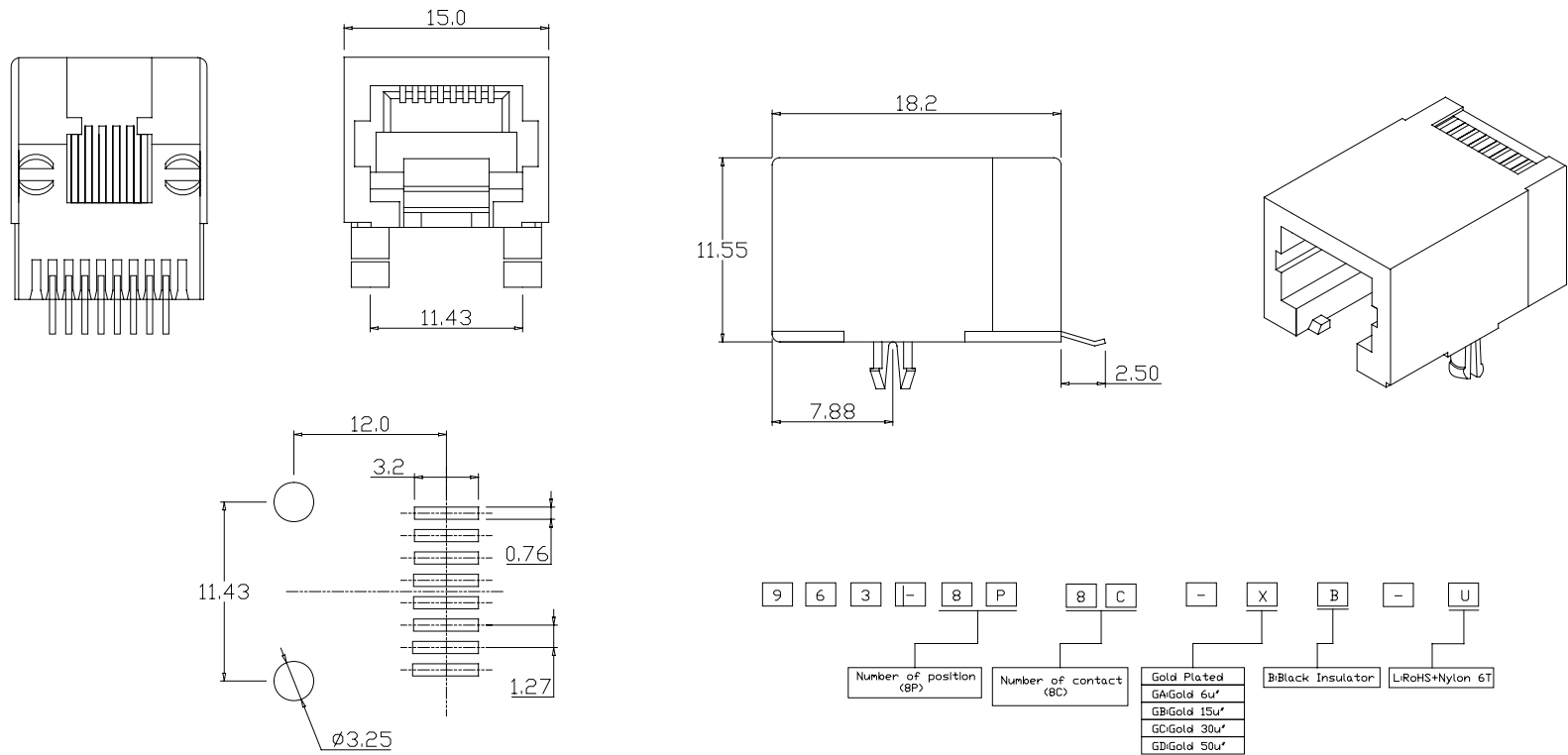
Recommended PCB Layout (PCB TOLERANCE \pm 0.05)
